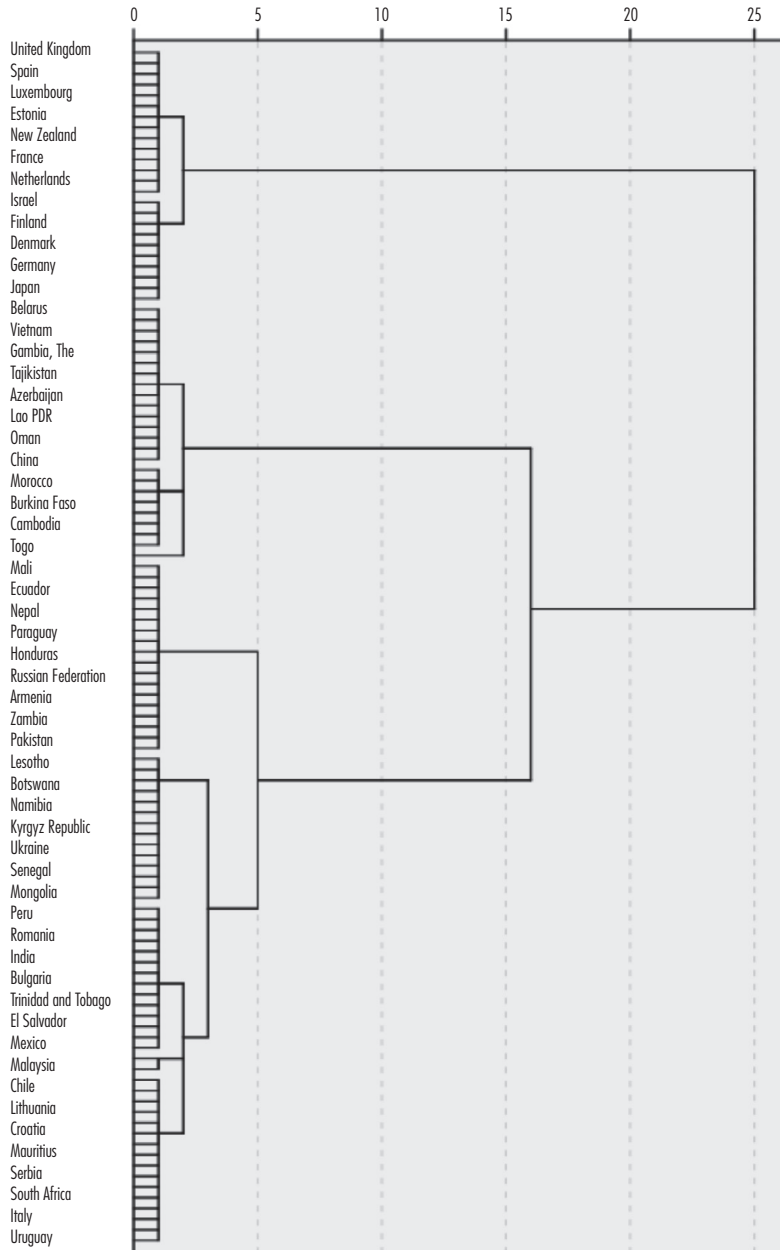
Figure 2. Dendrogram
